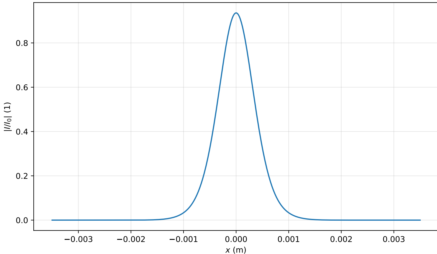
Intensity profile I(x, y = 0, z = 1.592m)/I_0 , P_{in}=0.5P_{cr} , artificial time
